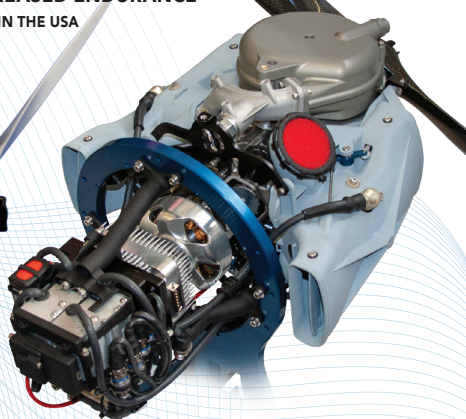
NW-88 TWIN-CYLINDER MULTI-FUEL ENGINE 40.8-74.8 kg Weight Class*
